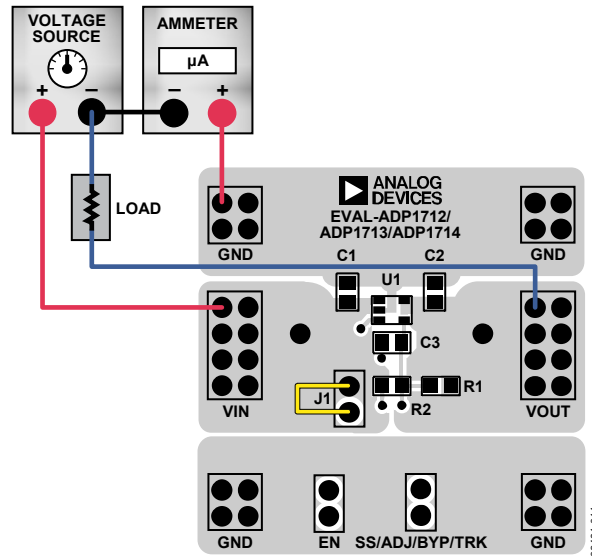
Figure 11. Ground Current Measurement
